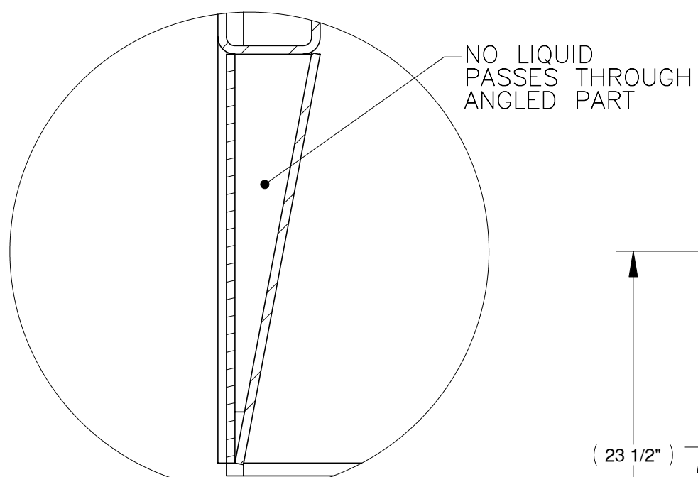
DETAIL 1 SCALE 1 : 4 ANGLE/FLAT BAR WELDMENT
